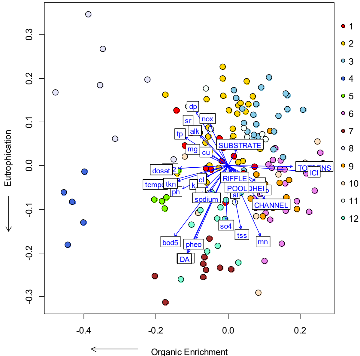
Figure 44 - Macroinvertebrate sites plotted by non-metric multidimensional scaling scores (the first two axes) performed on the distance matrix generated from large river macroinvertebrate data.
