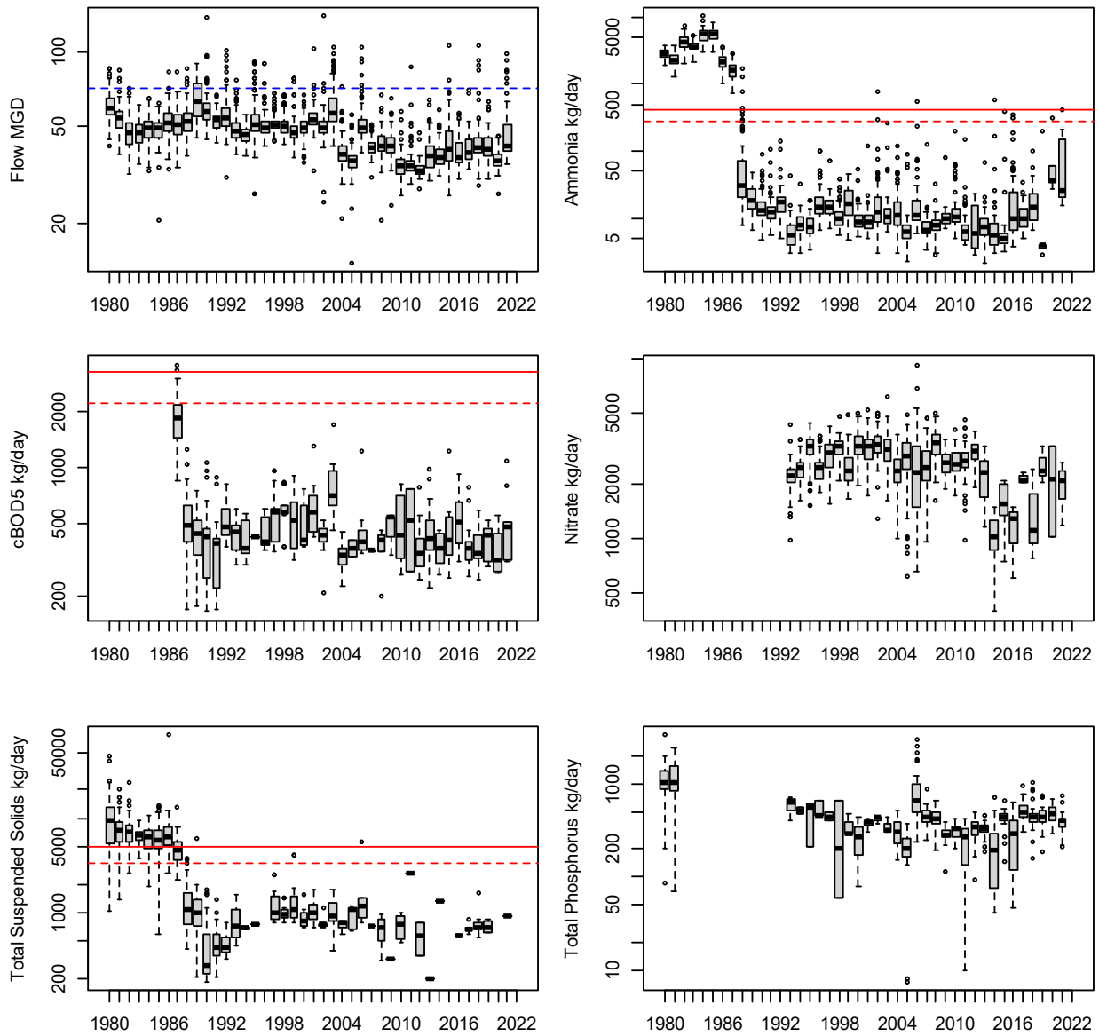
Figure 21 - Pollutant loads from the Dayton facility.
