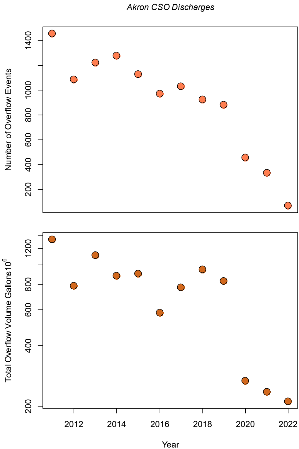
Figure 27 – Volumes of combined sewer overflows (CSO) reported by City of Akron.
