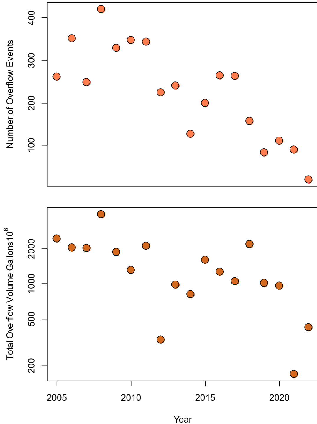
Figure 26 – Columbus combined sewer overflow discharges.
