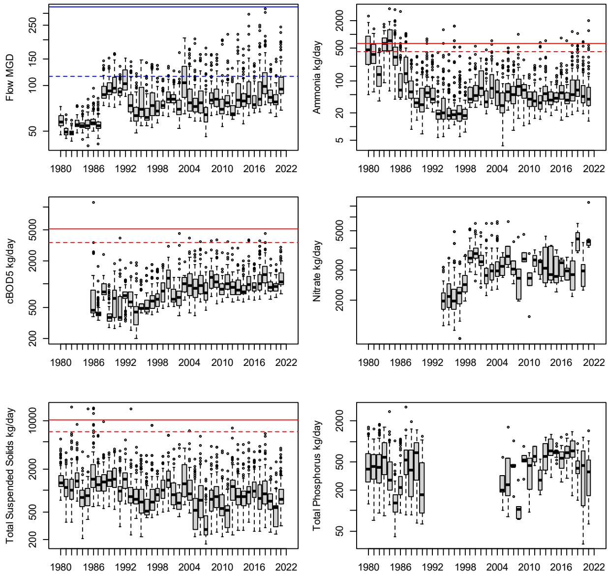
Figure 20 - Pollutant loads from the Columbus Southerly facility.
