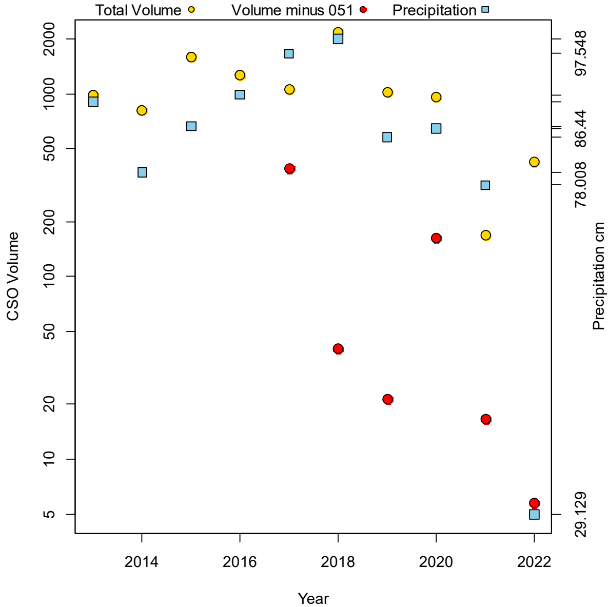
Figure 25 - Volumes of combined sewer overflows (CSO) reported by City of Columbus.
