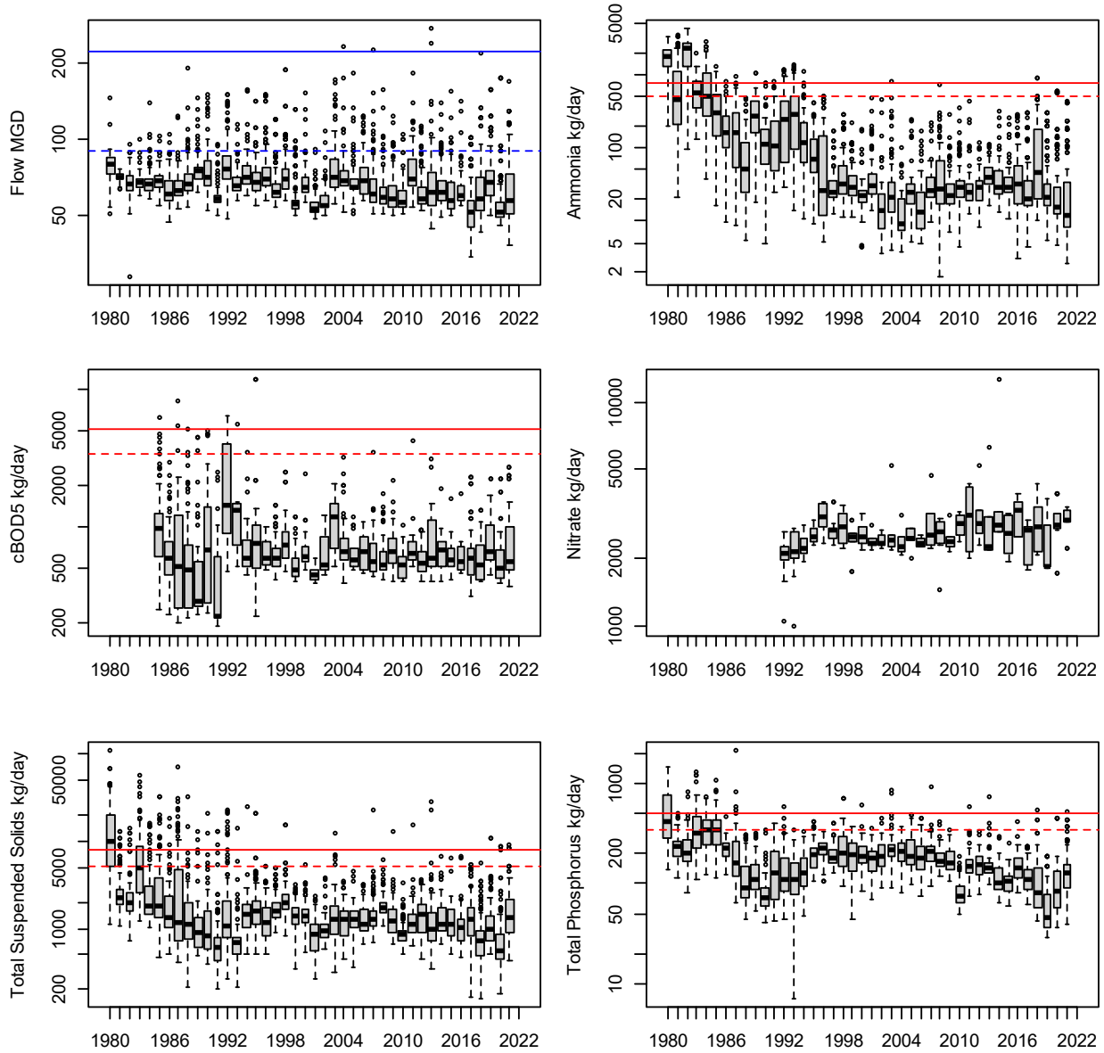
Figure 18 - Pollutant loads from the Akron facility.
