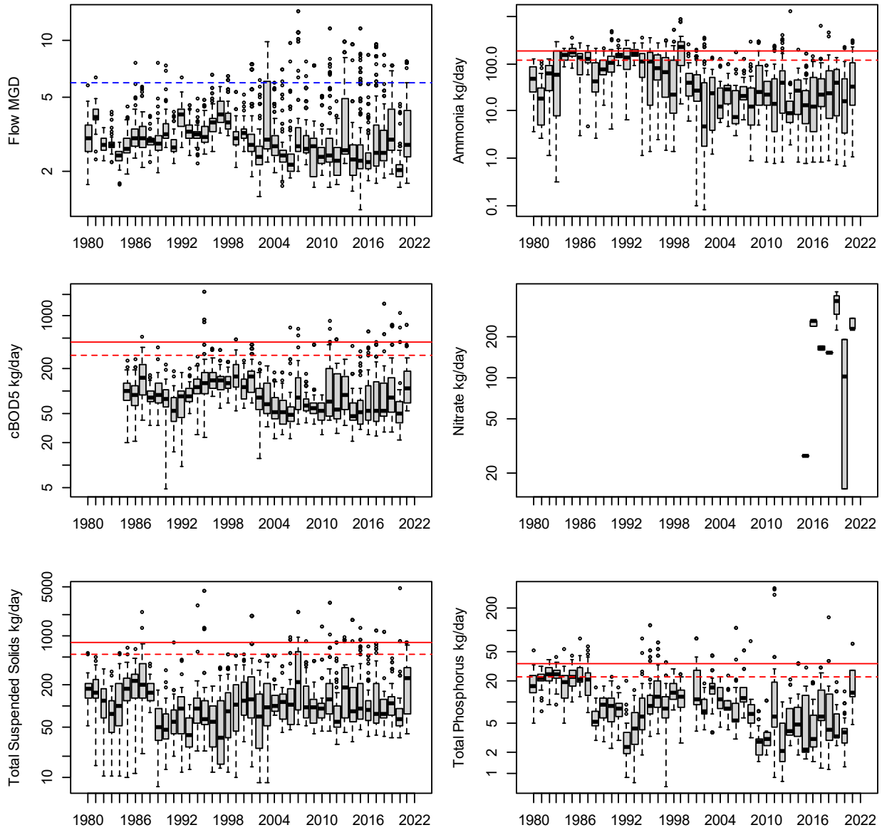
Figure 22 - Pollutant loads from the Defiance facility.
