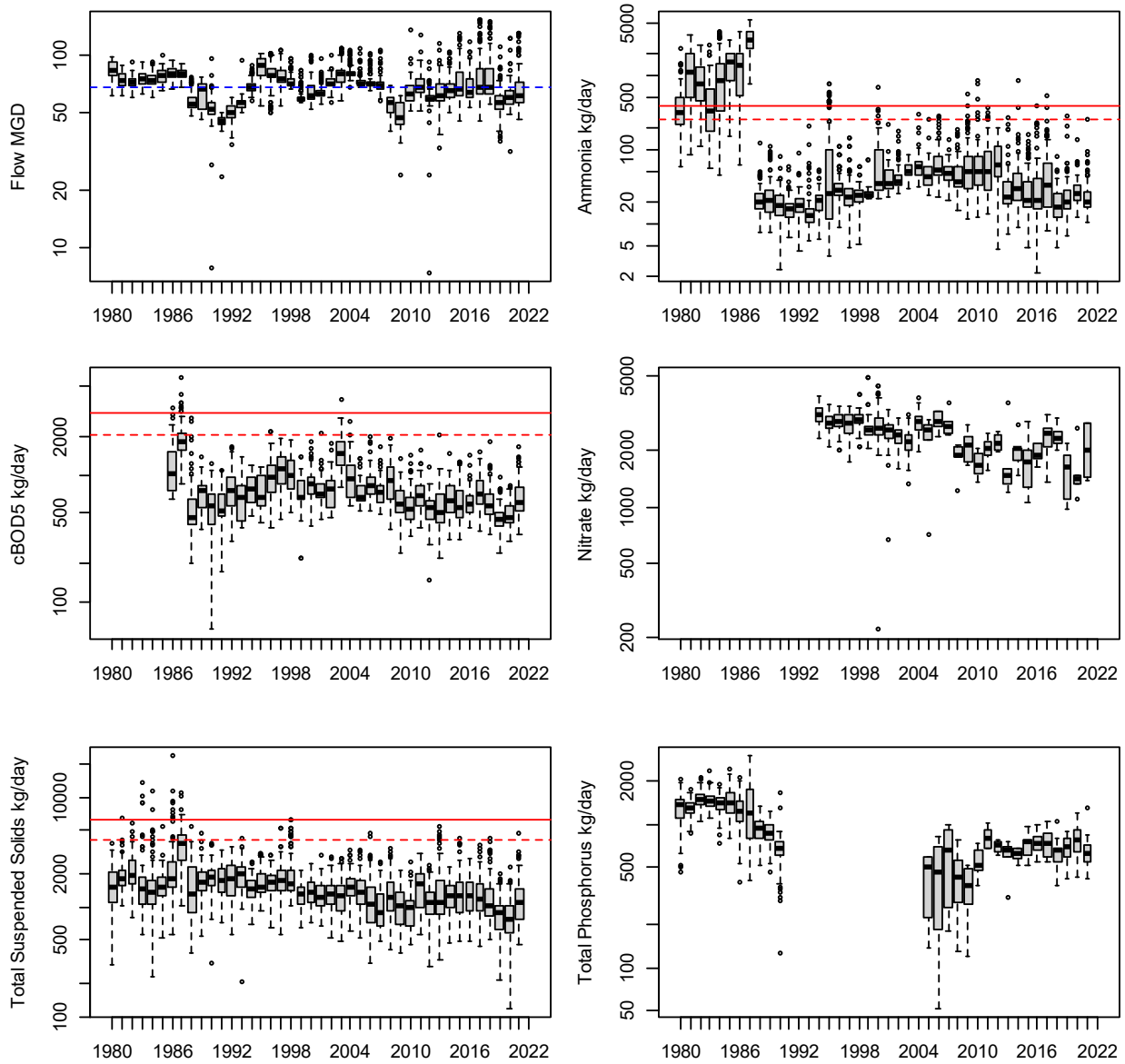
Figure 19 - Pollutant loads from the Jackson Pike facility.
