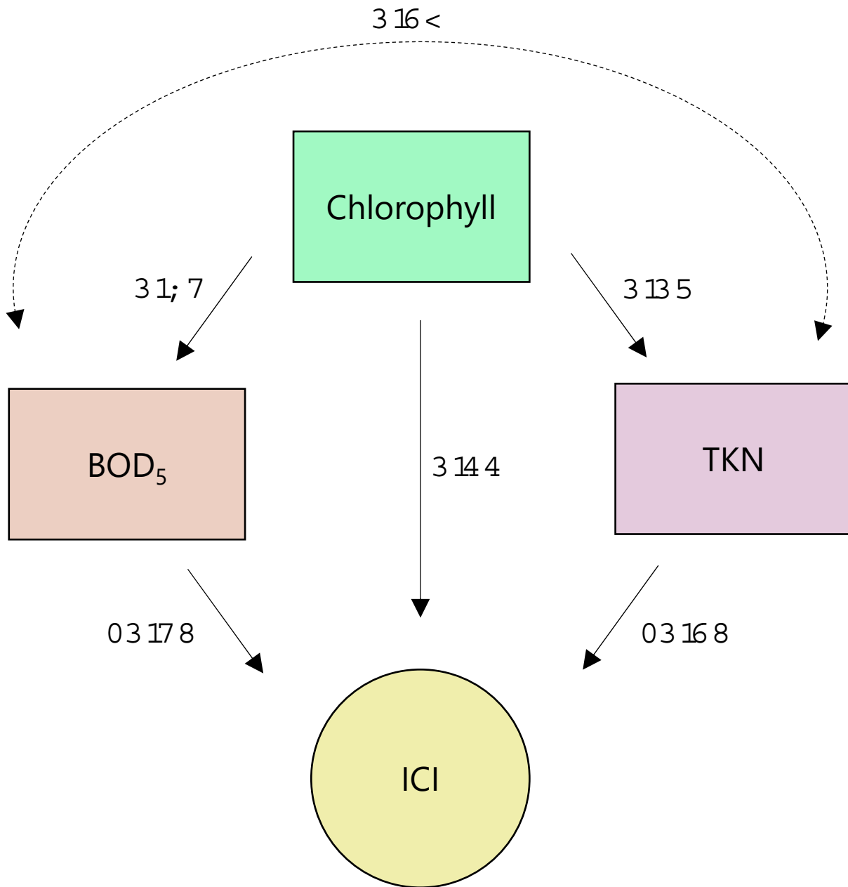
Figure 43 - A structural equation model linking ICI scores to BOD 5 , TKN and sestonic chlorophyll concentrations.
