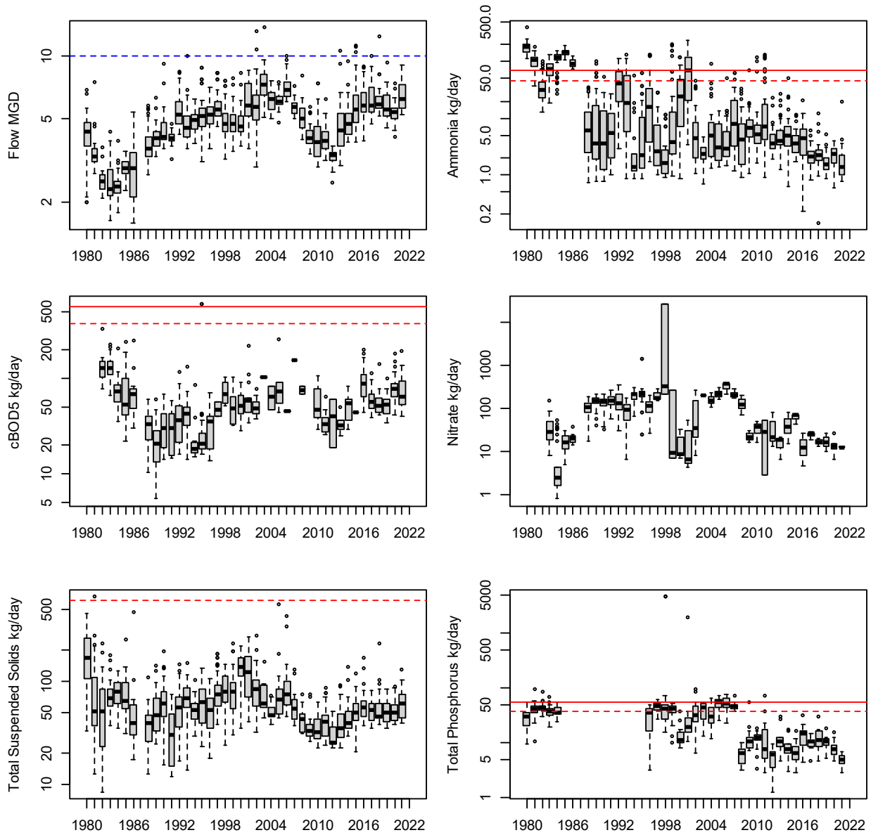
Figure 23 - Pollutant loads from the Sugar Creek (Little Miami River) facility.
