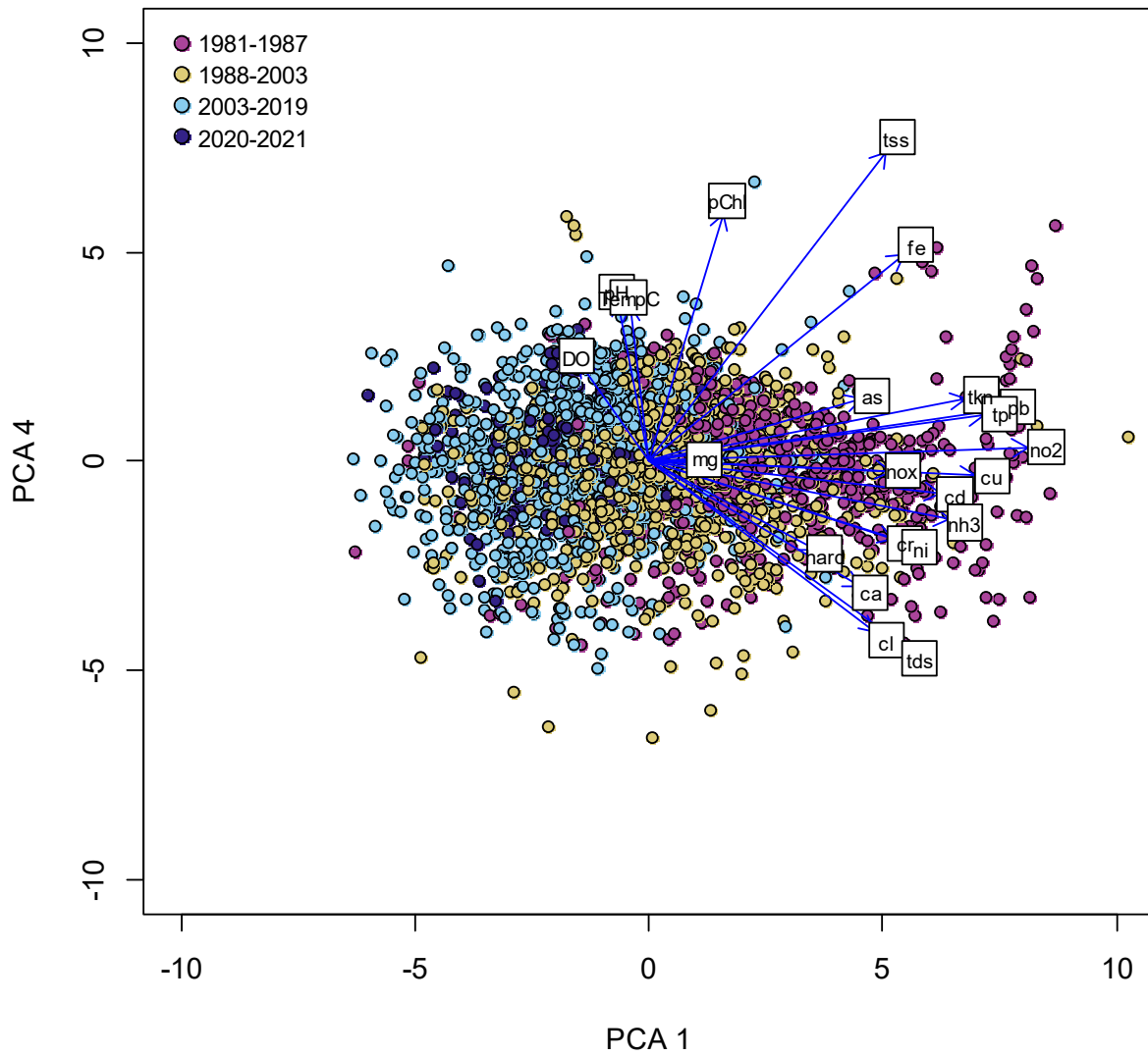
Figure 8 - A biplot showing the first and fourth axes from a principal components analysis (PCA) of water chemistry data collected from large rivers in Ohio, 1981-2021.
