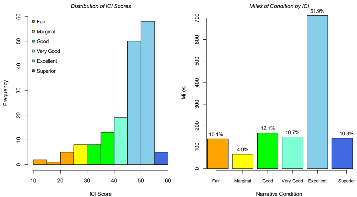
Figure 42 - Distributions of ICI scores color-coded by narrative class, and the number of assessed miles grouped by and color-coded to narrative condition class.
