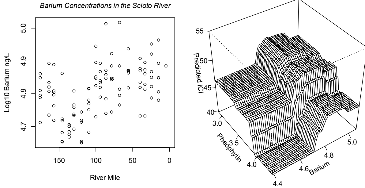
Relationship between barium, pheophytin, and modeled Invertebrate Community Index scores (from boosted regression).
